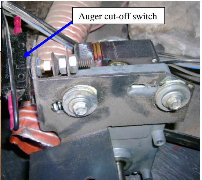
New Auger Motor on old bracket with spacers
